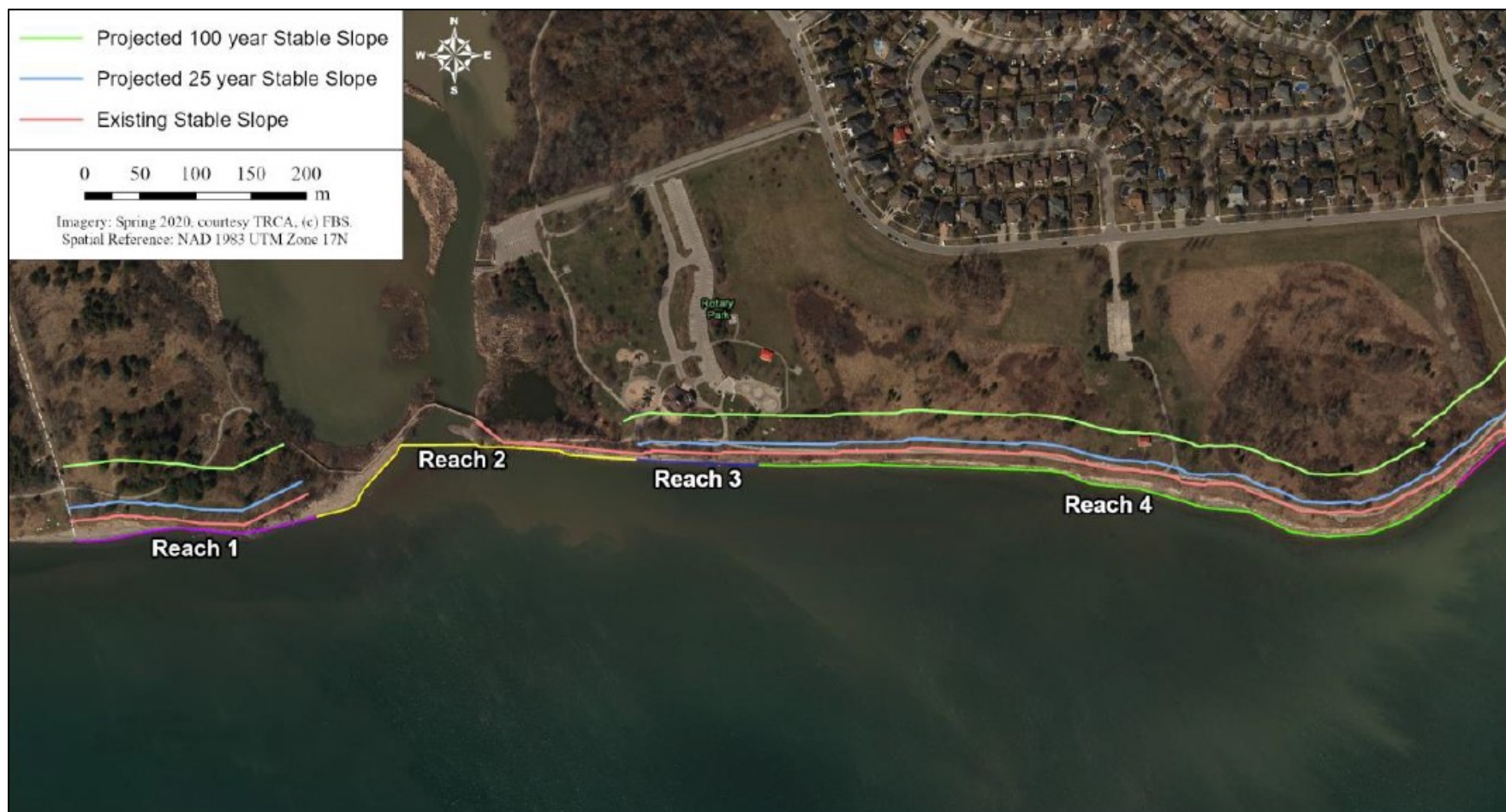
Figure 29. Long-term stable slope projections for Reaches 1-4. Source: Baird, 2023
