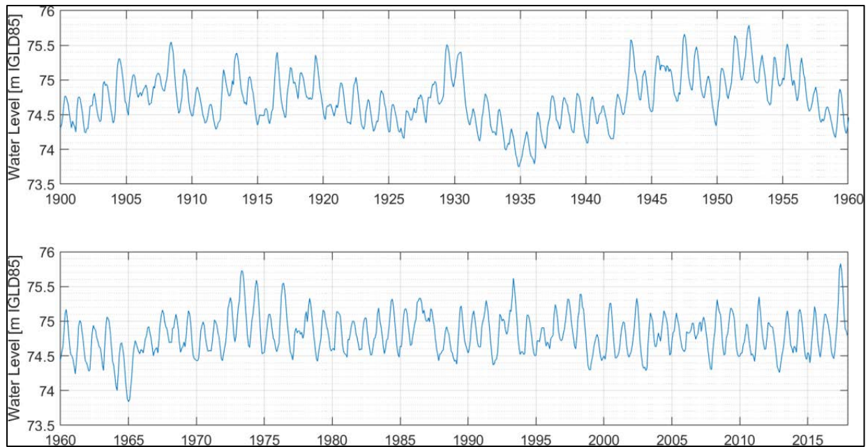
Figure 14. Water levels in Lake Ontario before regulation (top) and after regulation (bottom). Source: Baird, 2021.
