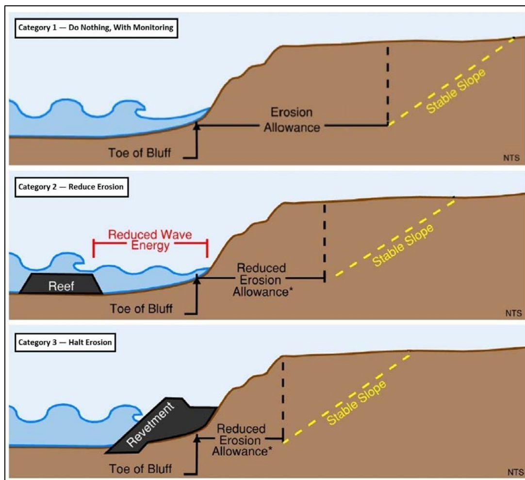
Figure 28. Three categories of designs for alternative development. The total amount of erosion and land loss decreases with Category 2 and 3 approaches. Source: Baird, 2023.
