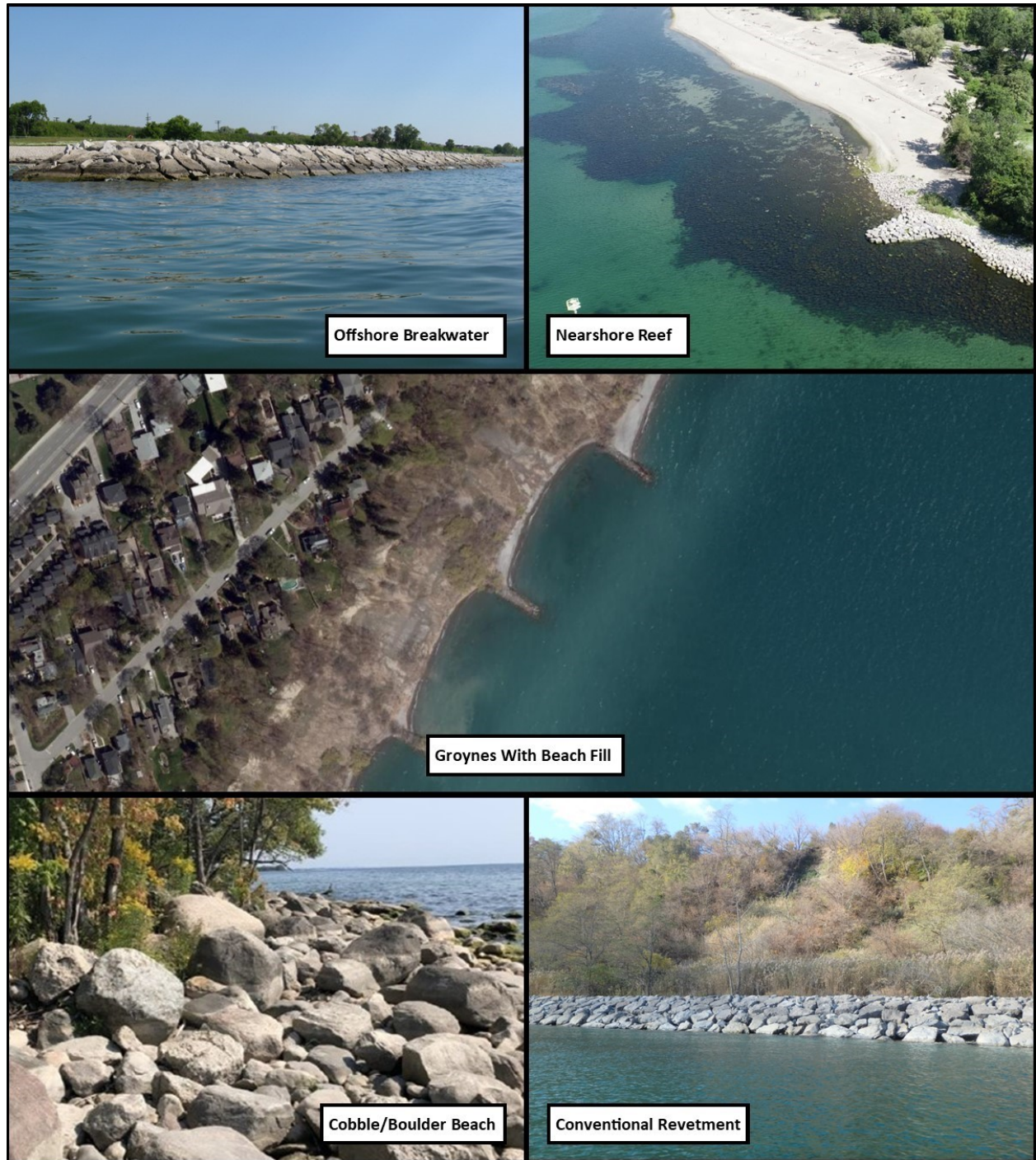
Figure 30. Examples of proposed preliminary alternatives from on-site and off-site examples. Source: TRCA, various years.
